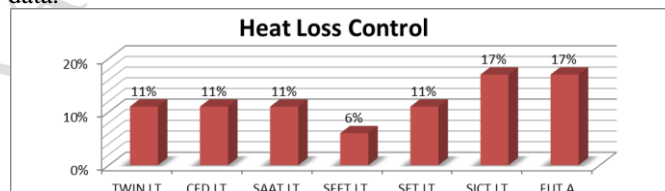
Figure 11: Heat Loss Control Measures Application in All the Lecture Theatres
