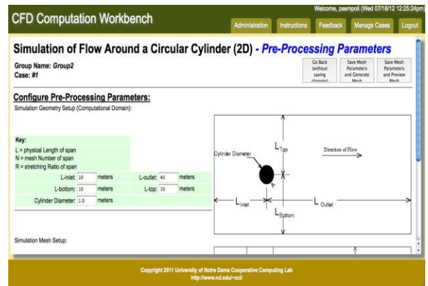
Figure 5: Mesh Parameters
